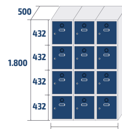
ECOC-40/3 COD: 84023 65,1kg · 1,08m 3
